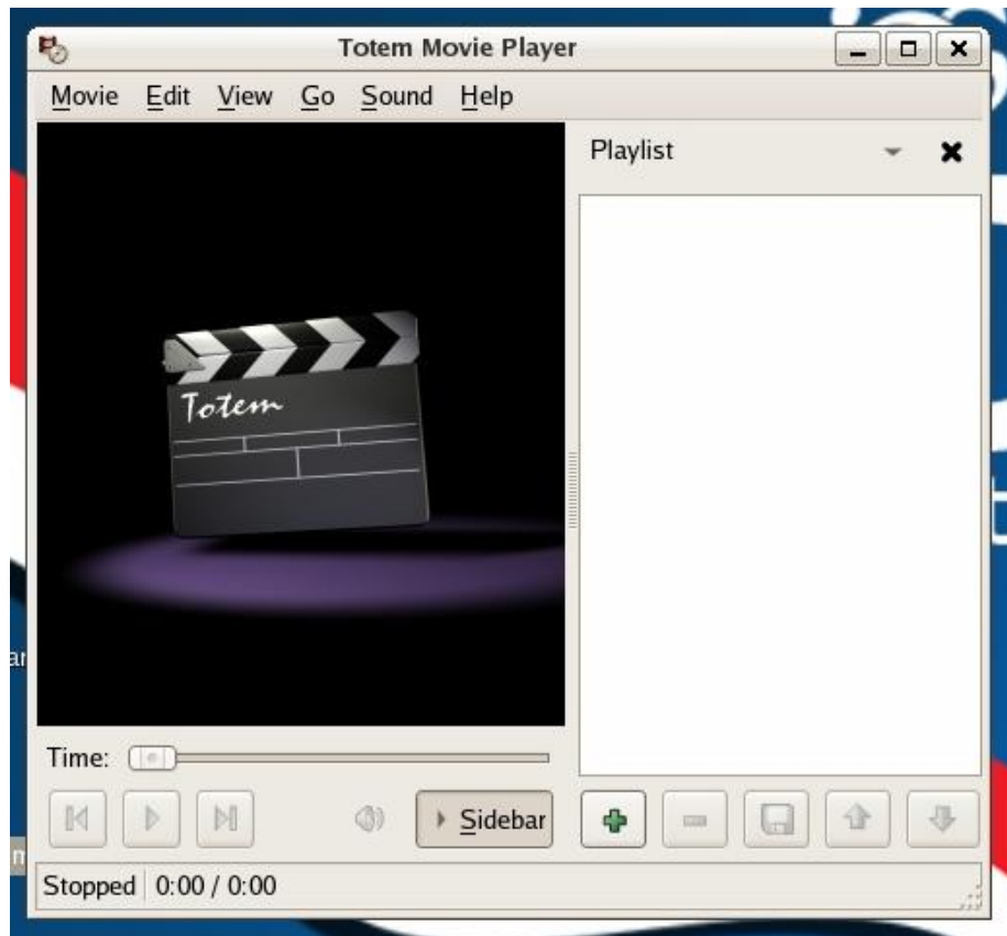
Gambar 4.4 Movie Player
